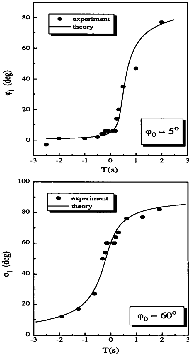
FIGURE 3 Two examples of measured (circles) and theoretical (solid line) values of \phi_1 at fixed light intensity and varying the depolarization time T . The theoretical curve is after a best-fit on the strength A and direction \phi_0 of the residual anisotropy. Different values of A and \phi_0 were obtained even for different spots of the same sample.
